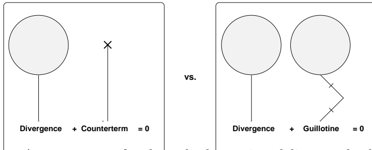
Fig. 3: A counterterm for the tadpole requires delicate order-by-order fine-tuning, and depends critically on the UV cutoff. By contrast, decapitation automatically generates contributions cancelling the tadpoles to all orders once the tree level deformation has been specified, and thus does not involve fine tuning.
